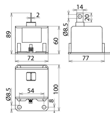
Dimension drawing DGPM 1 255 S
