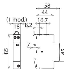
Dimension drawing DG TT 2P 5 275 NL
