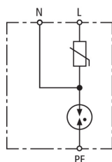
Basic circuit diagram DG TT 2P 5 275 NL
